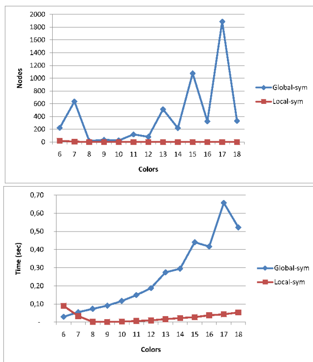
Figure 3: Node and Time curves of the two symmetry methods on random graph coloring where n = 30 and d = 0.5
