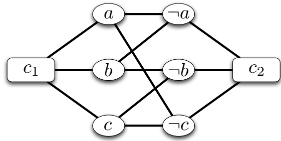
Figure 1: The graph G_{\mathcal{F}} corresponding to \mathcal{F}
